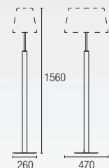
25-2825-21-82 + PAN 1 x E-27 Max. 100W Halogen - Fluorescent - LED
