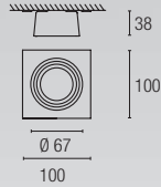
90-4350-14-14 1 x GU5.3 Max. 50W
