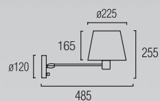
05-0381-81-AJ ■ 1 x E-27 Max. 60W Max. L=140mm Ø=60mm Halogen - Fluorescent
