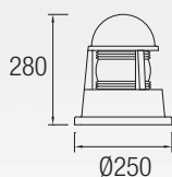
10-9645-Z5-M2 ■ E-27 max. 60W / max. L=180mm Halogen - Fluorescent - LED
