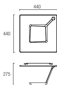
15-2412-BW-BW LED CREE 27W 2700 lm (N) 3000K
