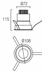
90-3475-14-14 LED CREE max. 8,8W 646 Lm lm 3000 K
