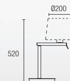
10-4696-81-82 + PAN 10-4696-Y2-82 + PAN 1 x E-27 Max. 60W Halogen - Fluorescent - LED
