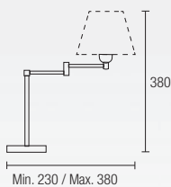
174-NS ■ + PAN 1 x E-27 Max. 60W Halogen - Fluorescent - LED
