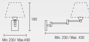
170-NS ■ + PAN 1 x E-27 Max. 60W Halogen - Fluorescent - LED
