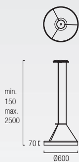
00-0001-BW-M3 (Standard) 00-0641-BW-M3 (Dimmable 1-10V) LED 22W 2.442 Lm (N) 3000K
