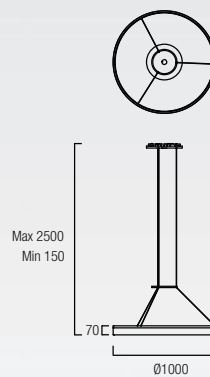
00-3642-BW-M3 (Standard) 00-3646-BW-M3 (Dimmable 1-10V) LED 36W 3986 Lm (N) 3000K
