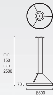
00-0002-BW-M3 (Standard) 00-0642-BW-M3 (Dimmable 1-10V) LED 31W 3.441 Lm (N) 3000 K
