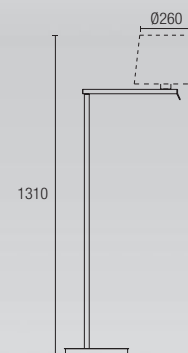
25-4696-81-82 + PAN 25-4696-Y2-82 + PAN 1 x E-27 Max. 100W Halogen - Fluorescent - LED
